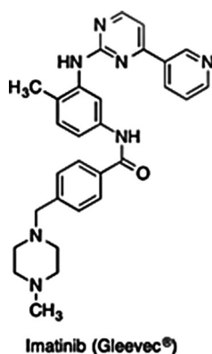
Figure 8. Imatinib.
