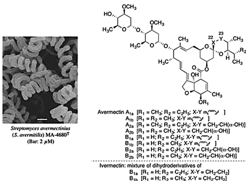
Figure 22. Avermectin.
